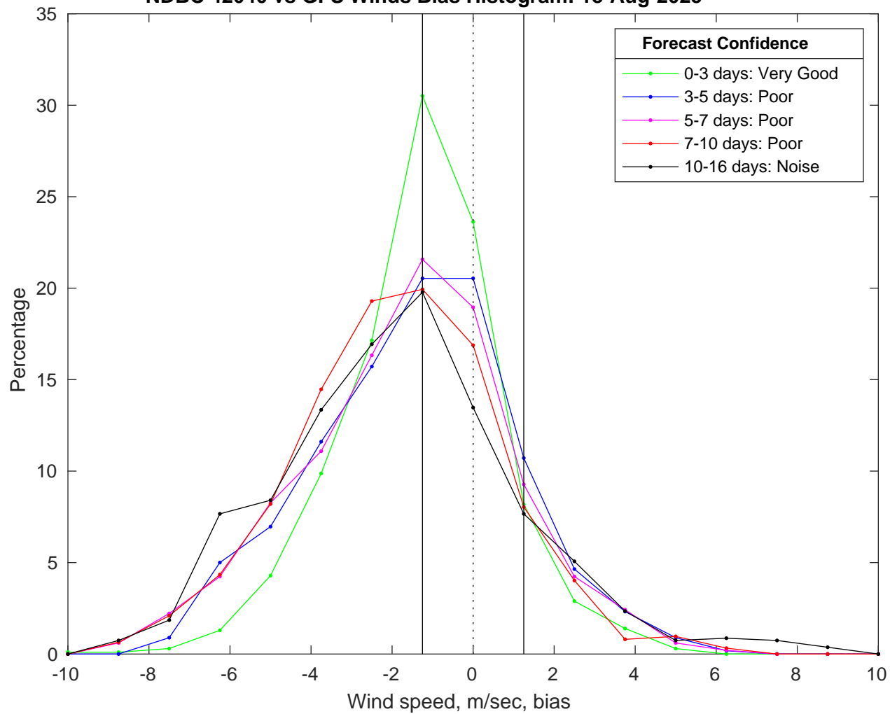
NDBC 42040 vs GFS Winds Bias Histogram: 18-Aug-2025
