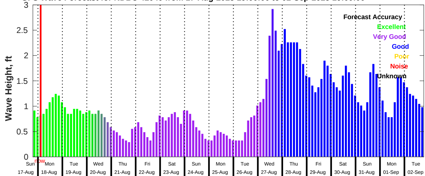
GFS Wave Forecast for NDBC 42040 from 17-Aug-2025 19:00:00 to 02-Sep-2025 19:00:00
