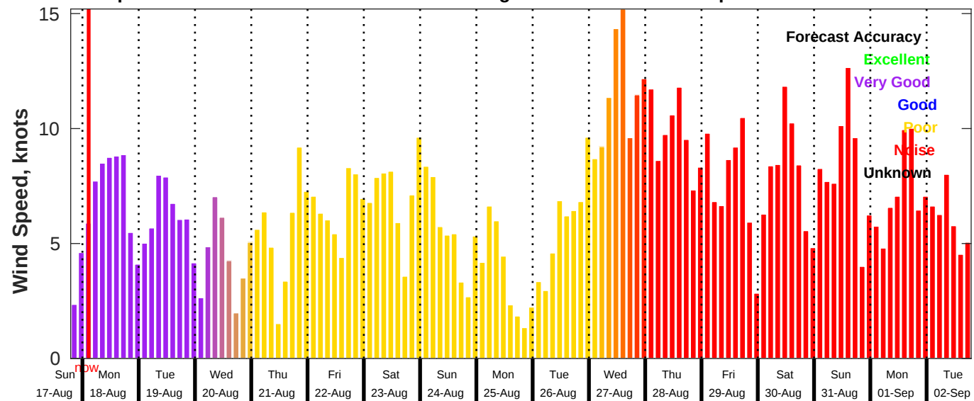
GFS Wind Speed Forecast for NDBC 42040 from 17-Aug-2025 19:00:00 to 02-Sep-2025 19:00:00
