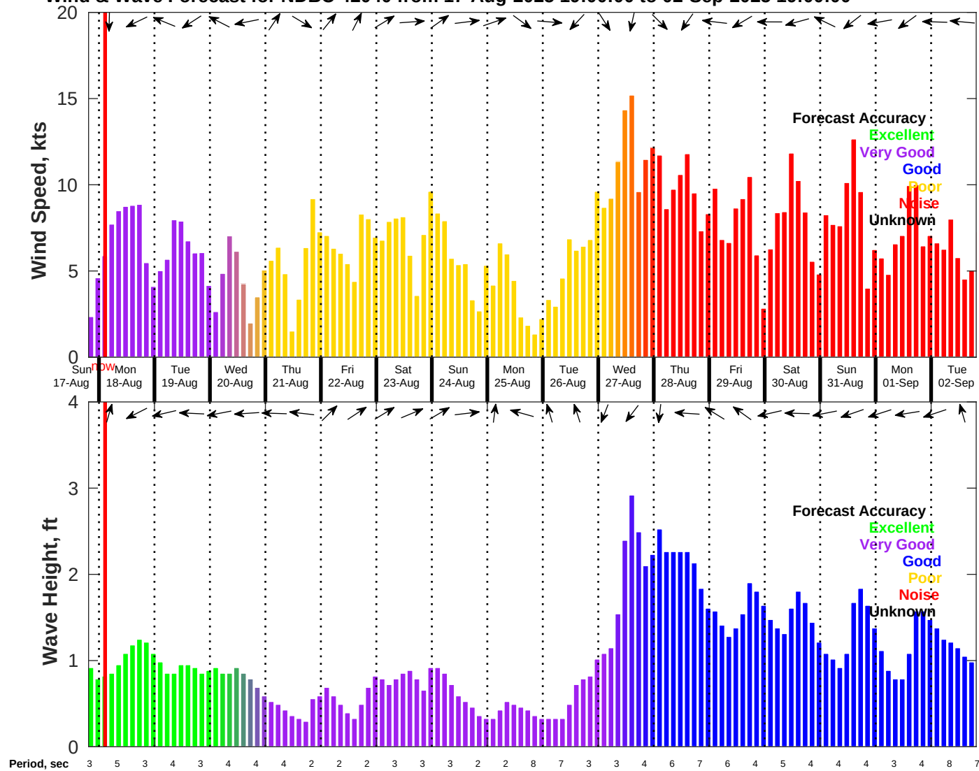
Wind & Wave Forecast for NDBC 42040 from 17-Aug-2025 19:00:00 to 02-Sep-2025 19:00:00
