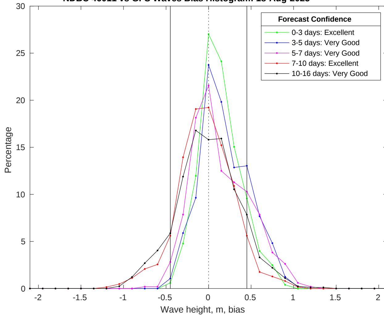
NDBC 46011 vs GFS Waves Bias Histogram: 18-Aug-2025
