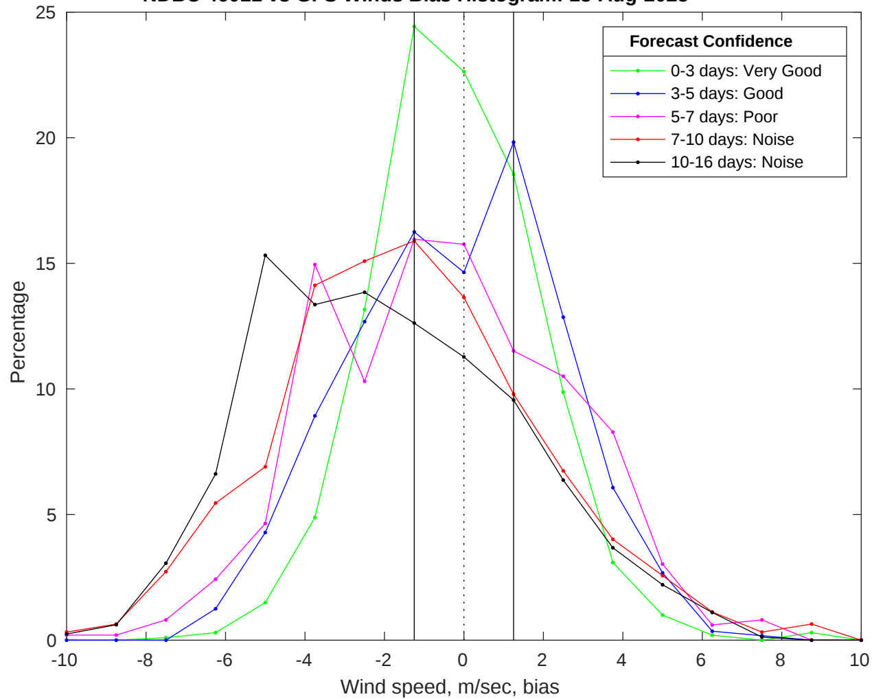
NDBC 46011 vs GFS Winds Bias Histogram: 18-Aug-2025
