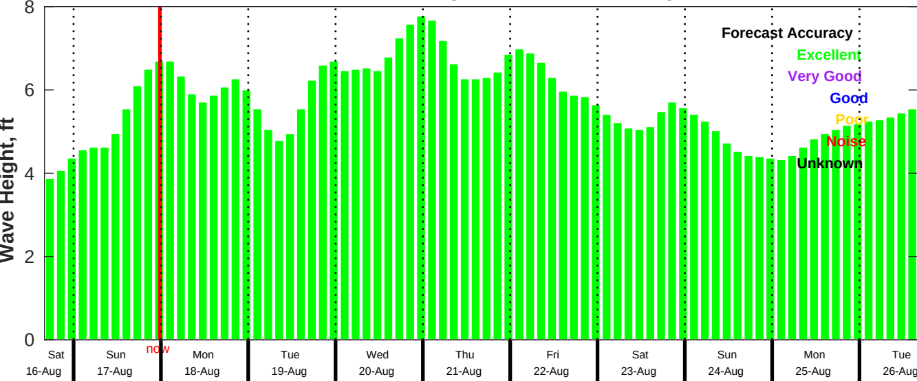
CMEMS Wave Forecast for NDBC 46011 from 16-Aug-2025 16:00:00 to 26-Aug-2025 16:00:00
