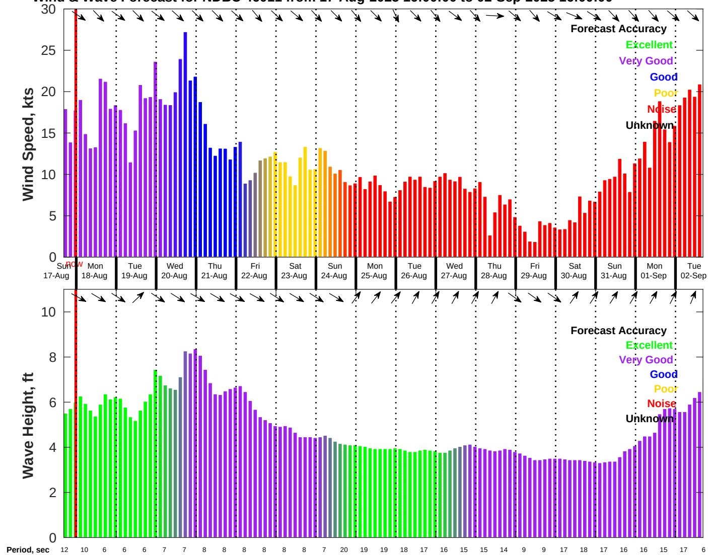
Wind & Wave Forecast for NDBC 46011 from 17-Aug-2025 16:00:00 to 02-Sep-2025 16:00:00
