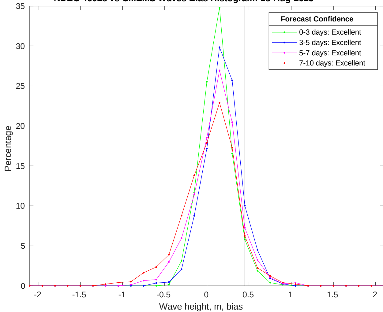
NDBC 46028 vs CMEMS Waves Bias Histogram: 18-Aug-2025
