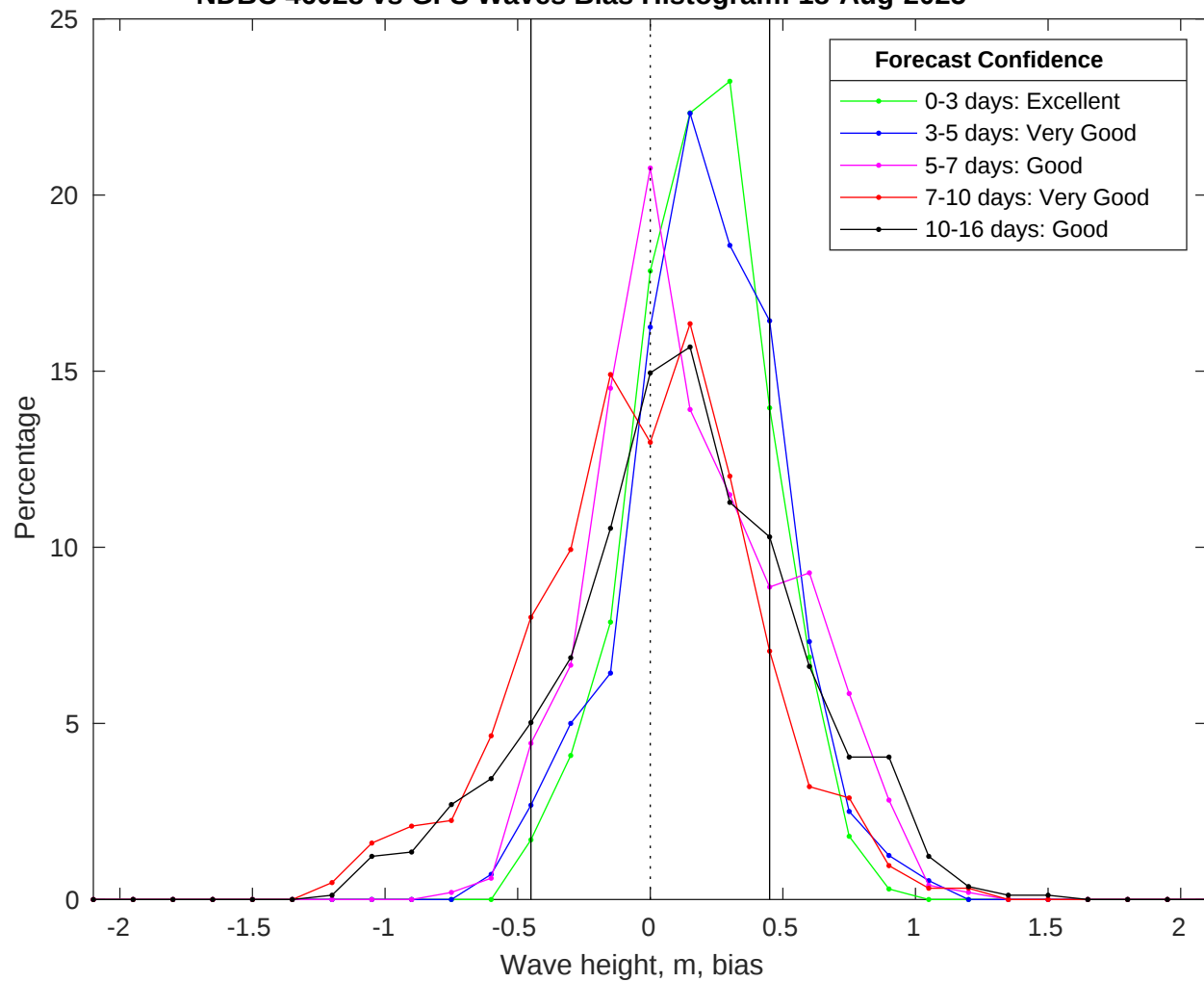
NDBC 46028 vs GFS Waves Bias Histogram: 18-Aug-2025
