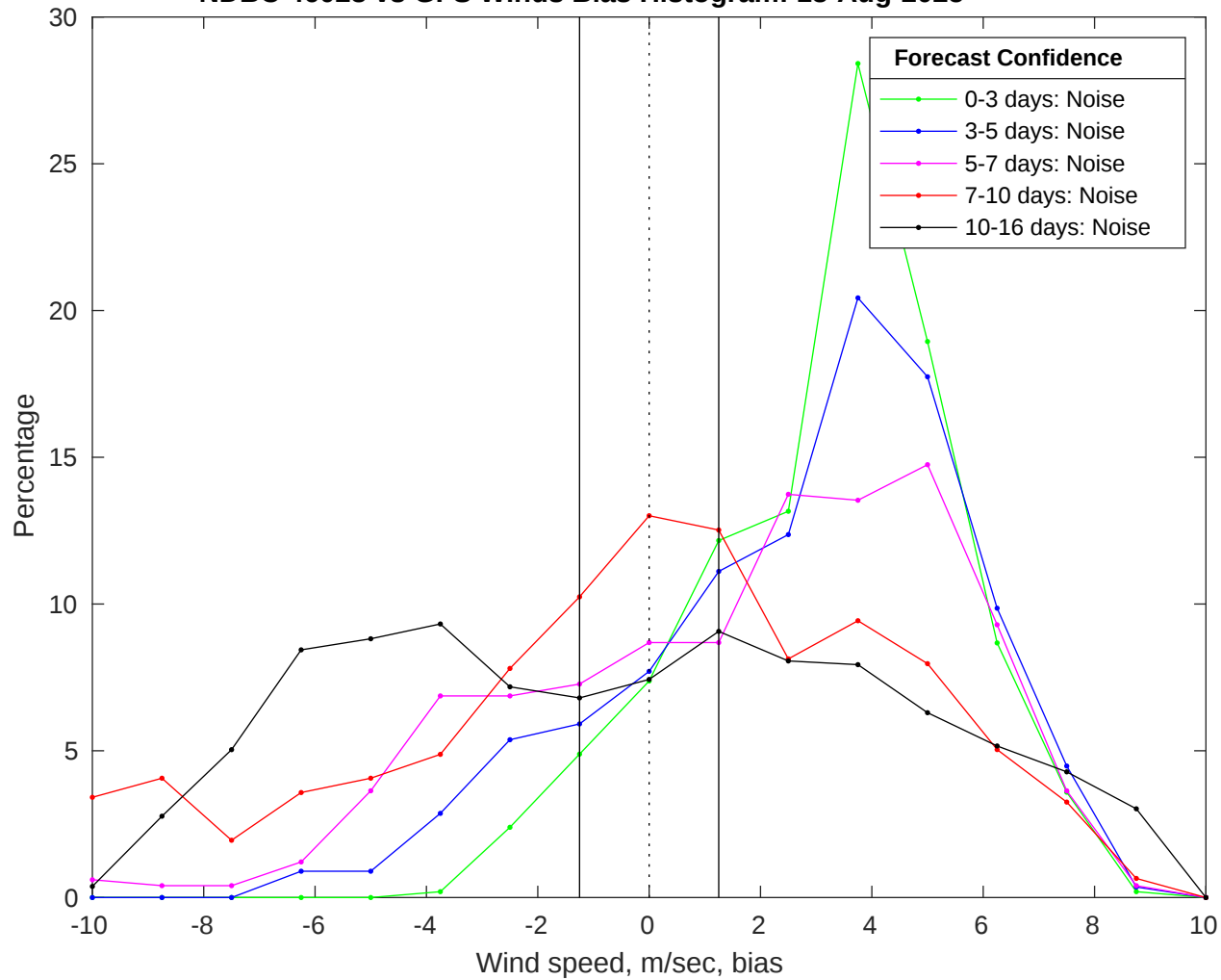
NDBC 46028 vs GFS Winds Bias Histogram: 18-Aug-2025
