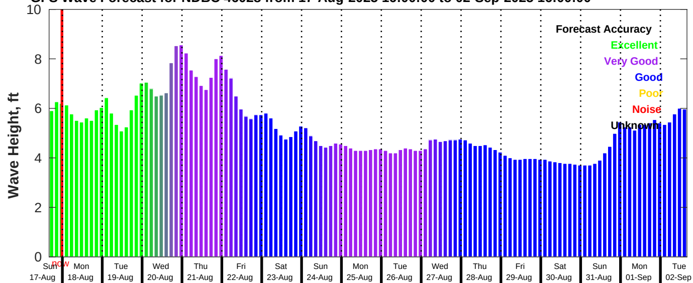
GFS Wave Forecast for NDBC 46028 from 17-Aug-2025 16:00:00 to 02-Sep-2025 16:00:00
