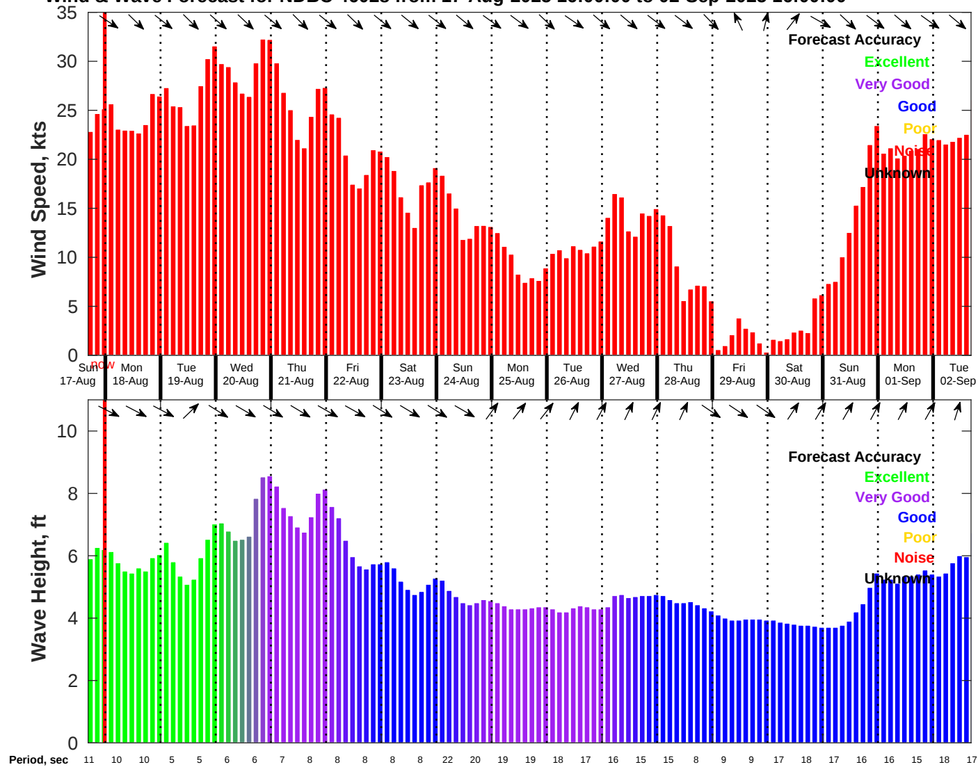
Wind & Wave Forecast for NDBC 46028 from 17-Aug-2025 16:00:00 to 02-Sep-2025 16:00:00
