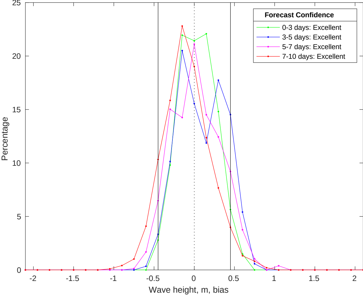
NDBC 46054 vs CMEMS Waves Bias Histogram: 18-Aug-2025
