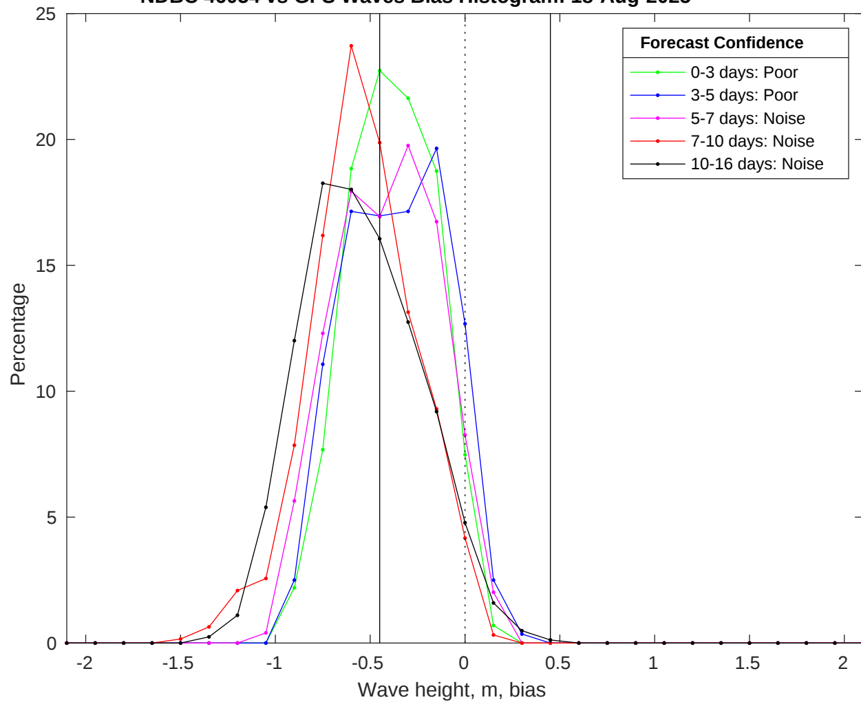
NDBC 46054 vs GFS Waves Bias Histogram: 18-Aug-2025
