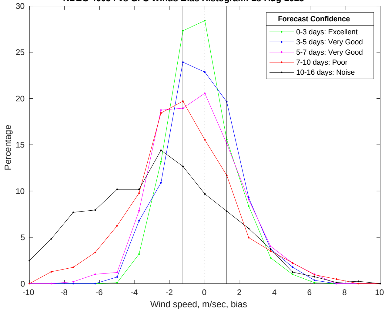
NDBC 46054 vs GFS Winds Bias Histogram: 18-Aug-2025
