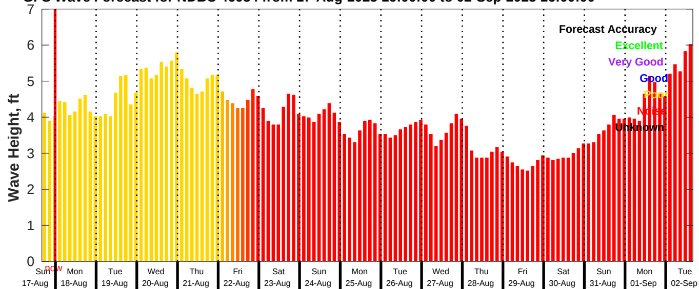
GFS Wave Forecast for NDBC 46054 from 17-Aug-2025 16:00:00 to 02-Sep-2025 16:00:00
