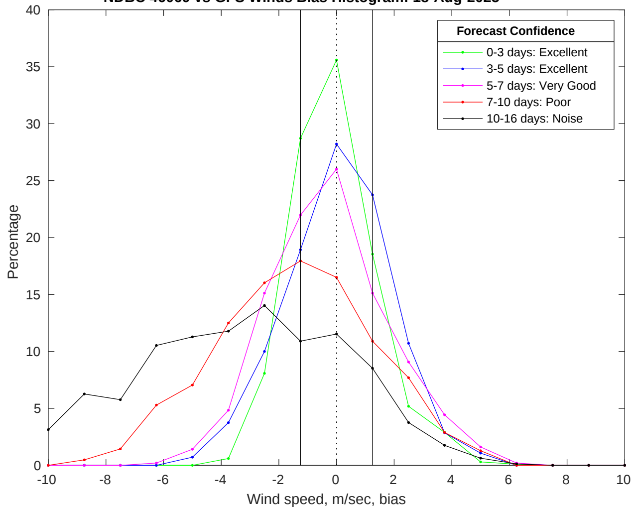
NDBC 46069 vs GFS Winds Bias Histogram: 18-Aug-2025
