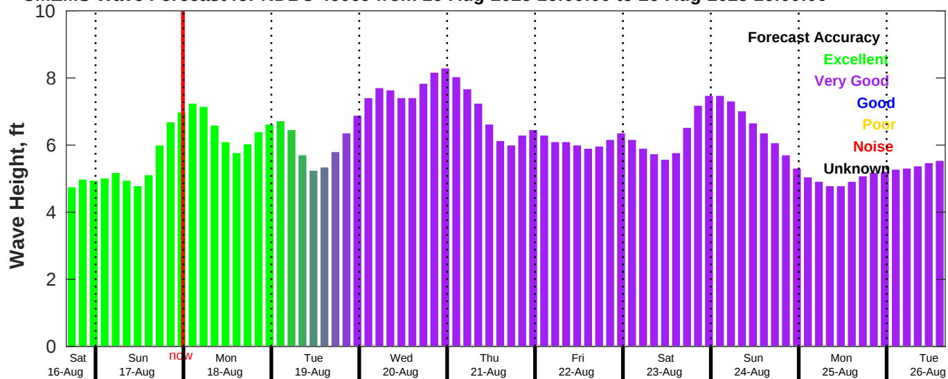
CMEMS Wave Forecast for NDBC 46069 from 16-Aug-2025 16:00:00 to 26-Aug-2025 16:00:00
