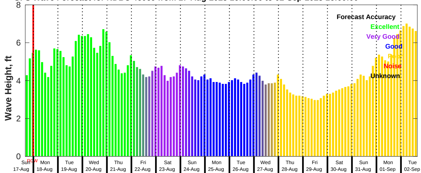
GFS Wave Forecast for NDBC 46069 from 17-Aug-2025 16:00:00 to 02-Sep-2025 16:00:00
