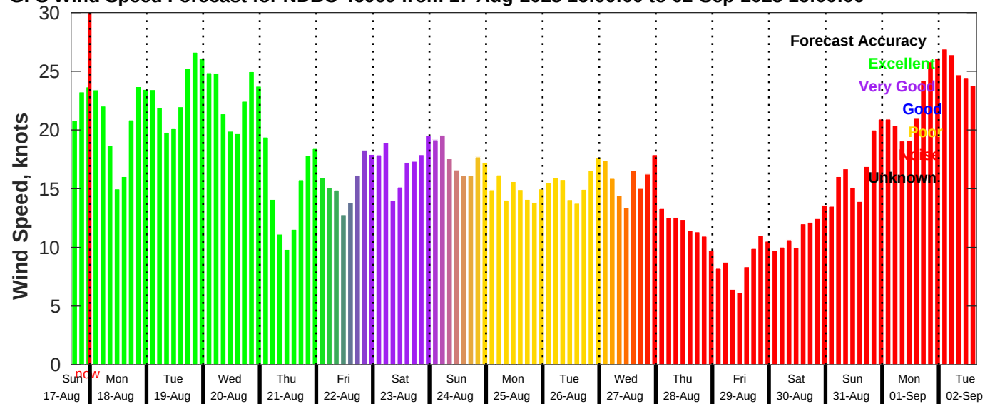
GFS Wind Speed Forecast for NDBC 46069 from 17-Aug-2025 16:00:00 to 02-Sep-2025 16:00:00
