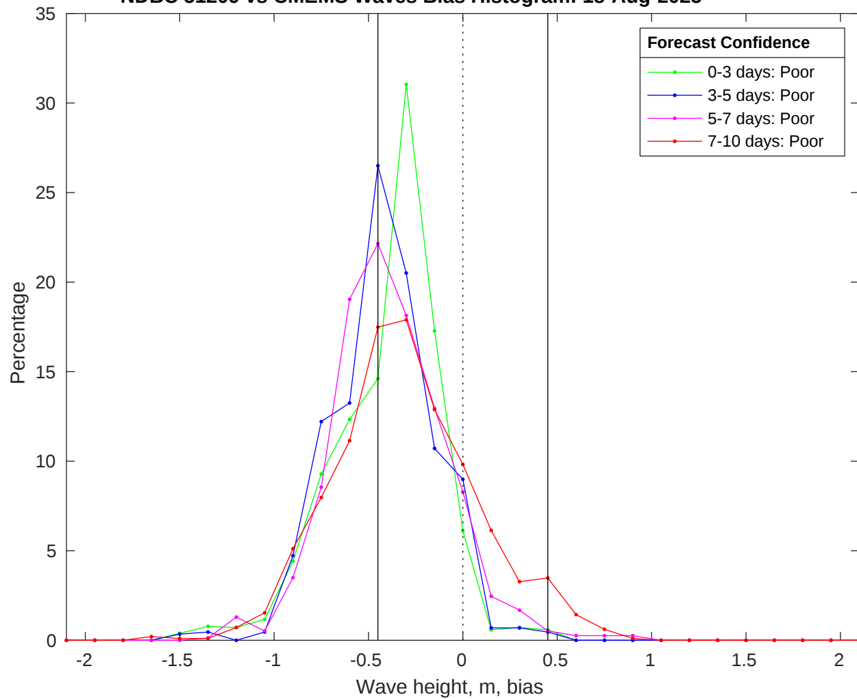
NDBC 51209 vs CMEMS Waves Bias Histogram: 18-Aug-2025
