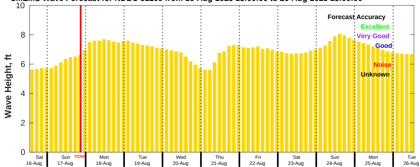
CMEMS Wave Forecast for NDBC 51209 from 16-Aug-2025 13:00:00 to 26-Aug-2025 13:00:00
