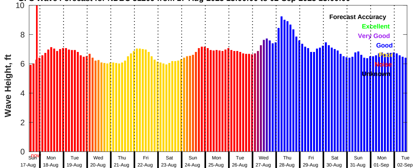
GFS Wave Forecast for NDBC 51209 from 17-Aug-2025 13:00:00 to 02-Sep-2025 13:00:00
