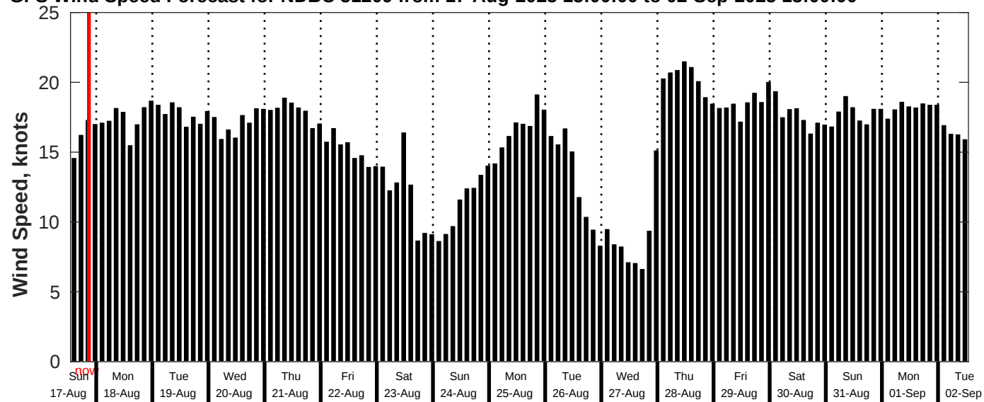
GFS Wind Speed Forecast for NDBC 51209 from 17-Aug-2025 13:00:00 to 02-Sep-2025 13:00:00
