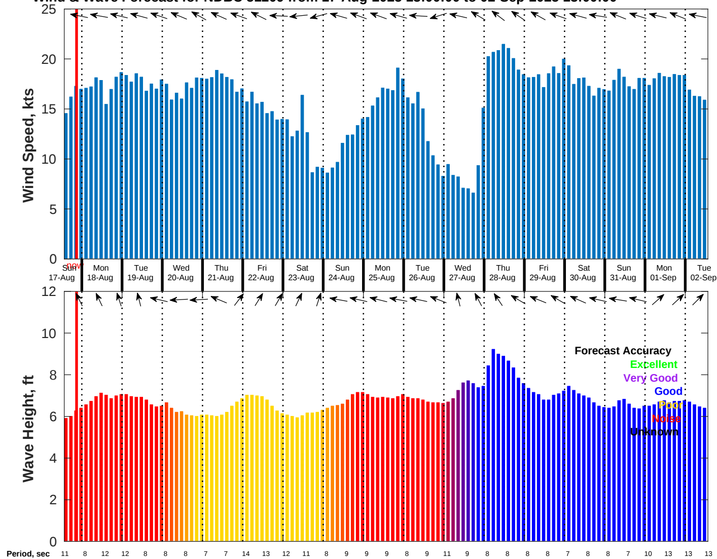
Wind & Wave Forecast for NDBC 51209 from 17-Aug-2025 13:00:00 to 02-Sep-2025 13:00:00
