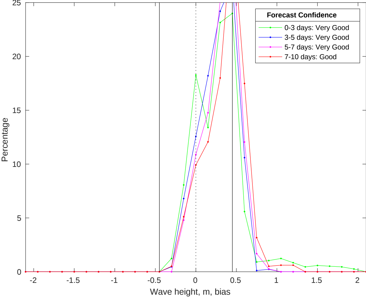
NDBC 51211 vs CMEMS Waves Bias Histogram: 18-Aug-2025
