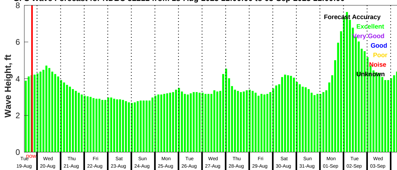
GFS Wave Forecast for NDBC 52211 from 18-Aug-2025 11:00:00 to 03-Sep-2025 11:00:00
