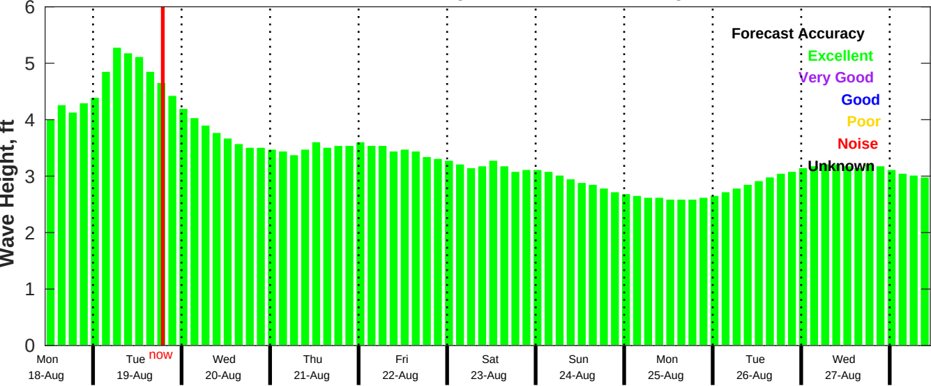
CMEMS Wave Forecast for NDBC 52213 from 17-Aug-2025 11:00:00 to 27-Aug-2025 11:00:00
