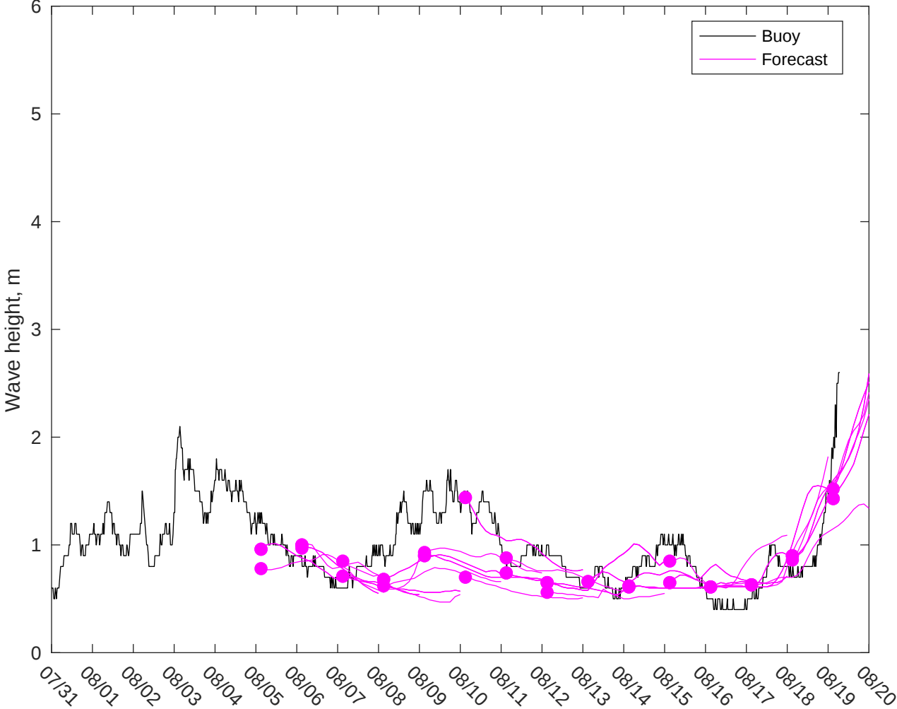
NDBC 41004 vs CMEMS Waves: 7 to 10 day forecast
