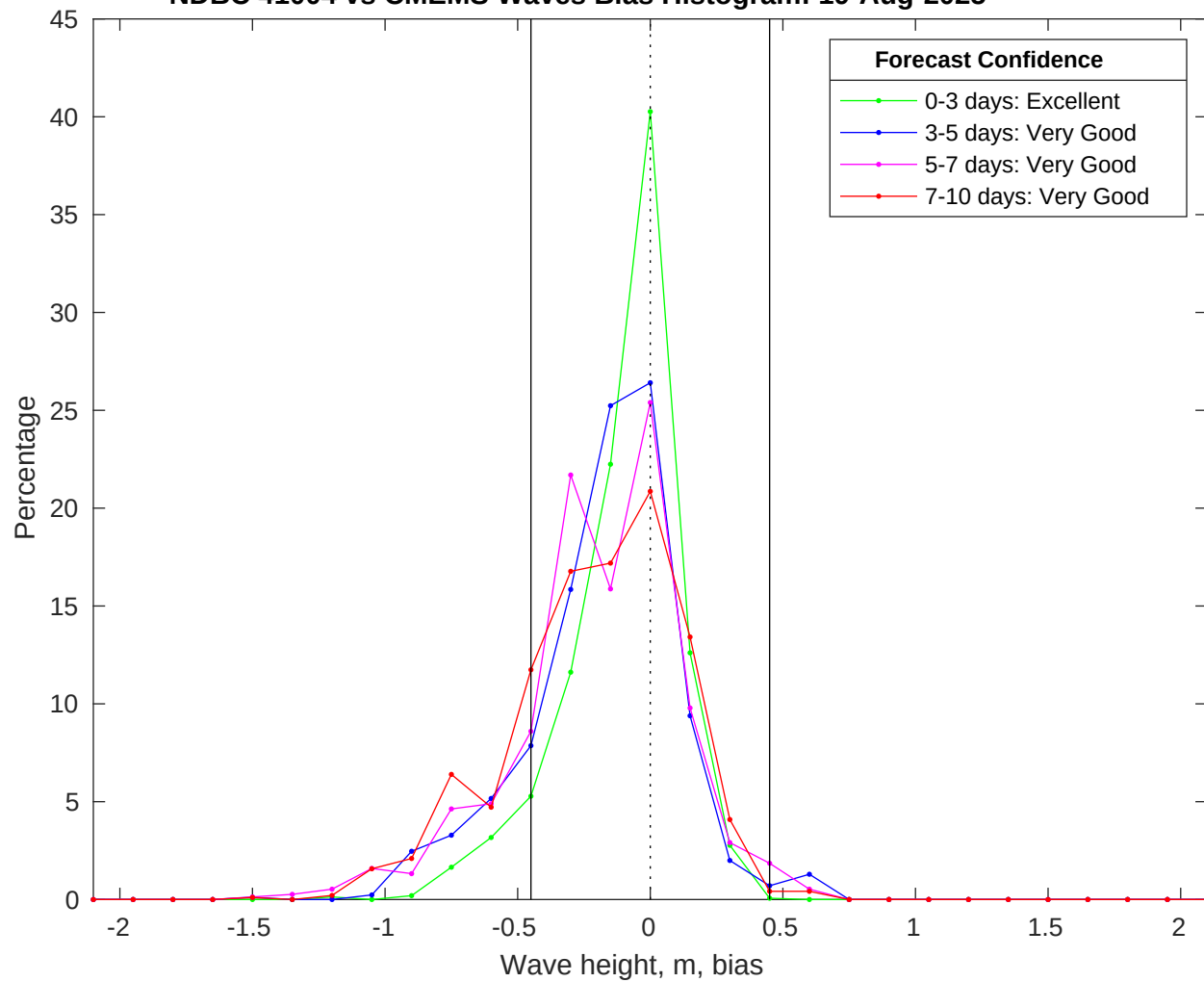
NDBC 41004 vs CMEMS Waves Bias Histogram: 19-Aug-2025
