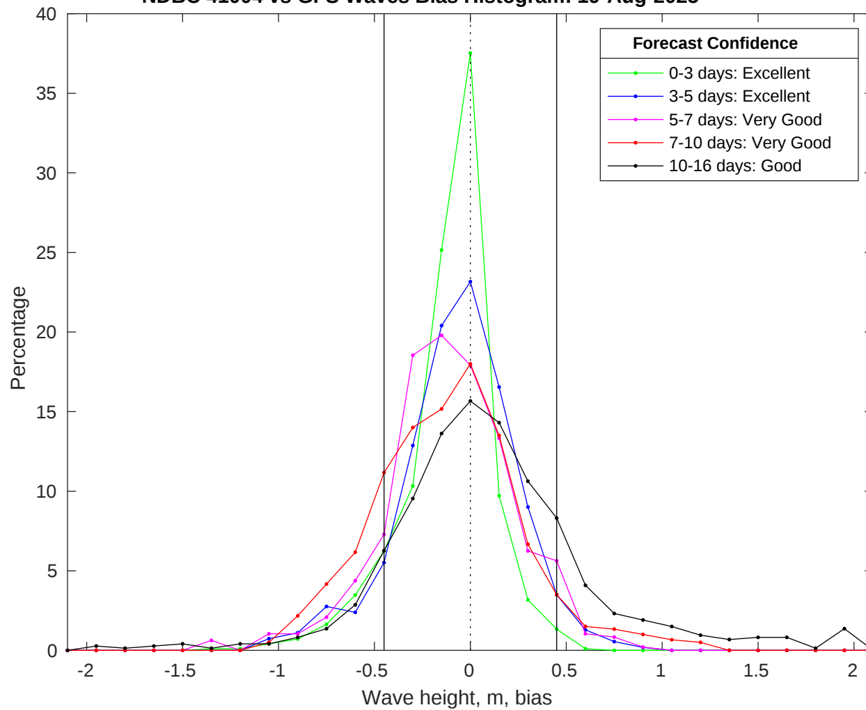
NDBC 41004 vs GFS Waves Bias Histogram: 19-Aug-2025
