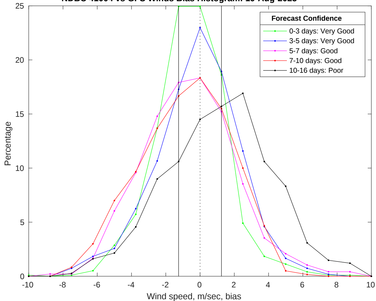
NDBC 41004 vs GFS Winds Bias Histogram: 19-Aug-2025
