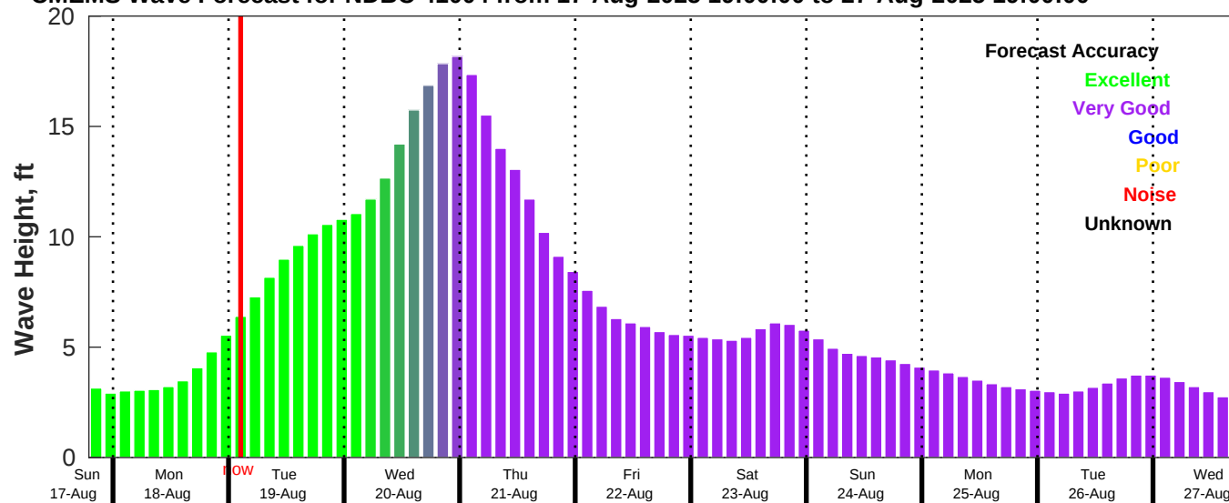
CMEMS Wave Forecast for NDBC 41004 from 17-Aug-2025 19:00:00 to 27-Aug-2025 19:00:00
