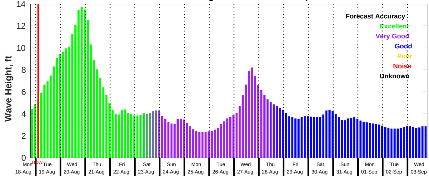
GFS Wave Forecast for NDBC 41004 from 18-Aug-2025 19:00:00 to 03-Sep-2025 19:00:00
