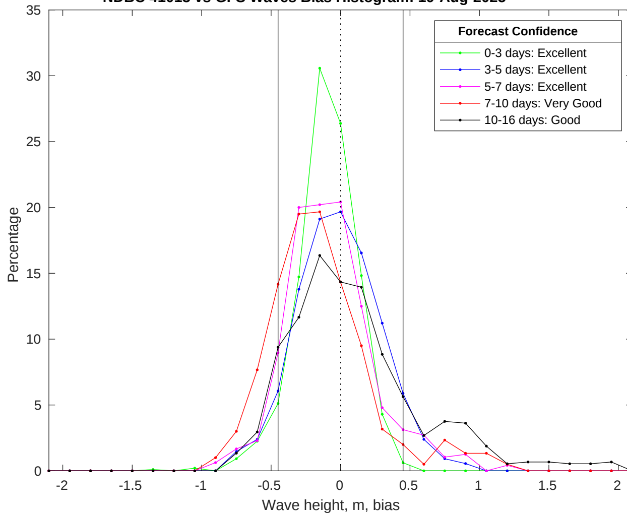
NDBC 41013 vs GFS Waves Bias Histogram: 19-Aug-2025
