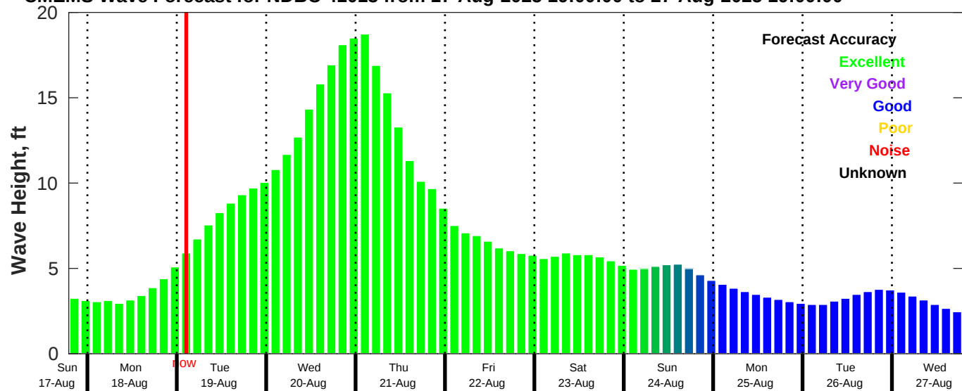
CMEMS Wave Forecast for NDBC 41013 from 17-Aug-2025 19:00:00 to 27-Aug-2025 19:00:00
