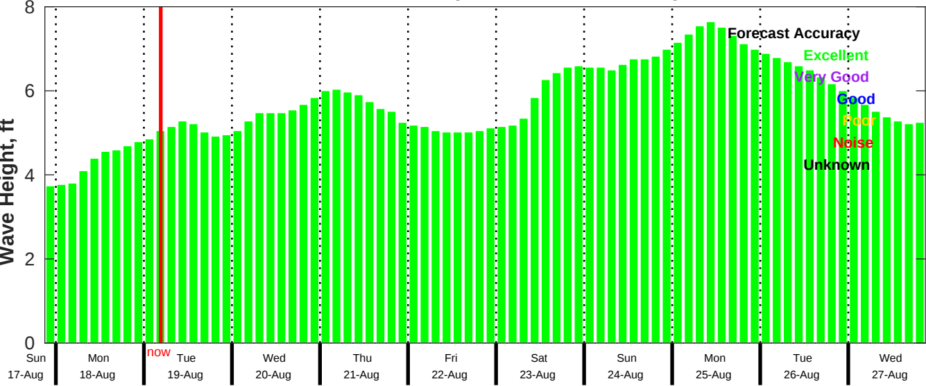
CMEMS Wave Forecast for NDBC 41040 from 17-Aug-2025 21:00:00 to 27-Aug-2025 21:00:00
