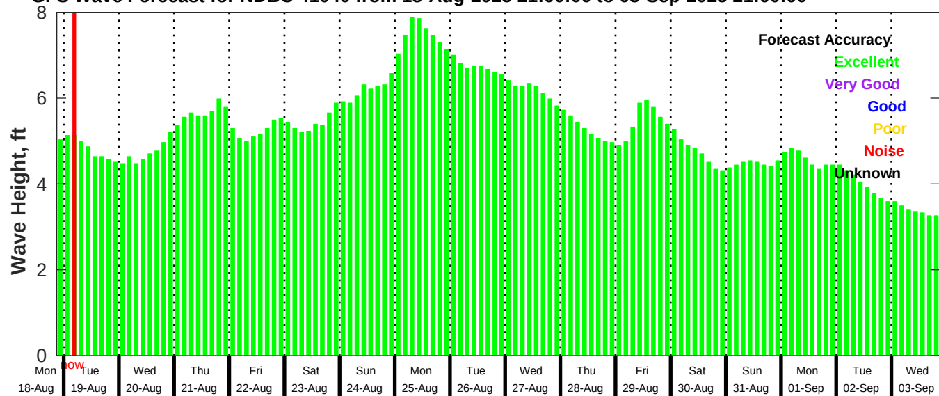
GFS Wave Forecast for NDBC 41040 from 18-Aug-2025 21:00:00 to 03-Sep-2025 21:00:00
