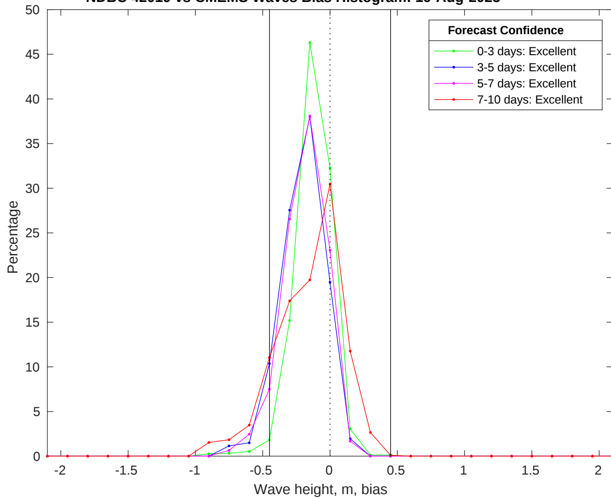
NDBC 42019 vs CMEMS Waves Bias Histogram: 19-Aug-2025
