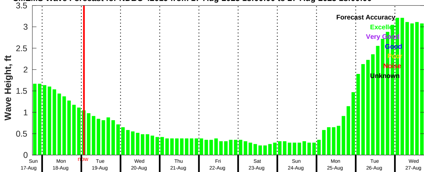
CMEMS Wave Forecast for NDBC 42019 from 17-Aug-2025 18:00:00 to 27-Aug-2025 18:00:00
