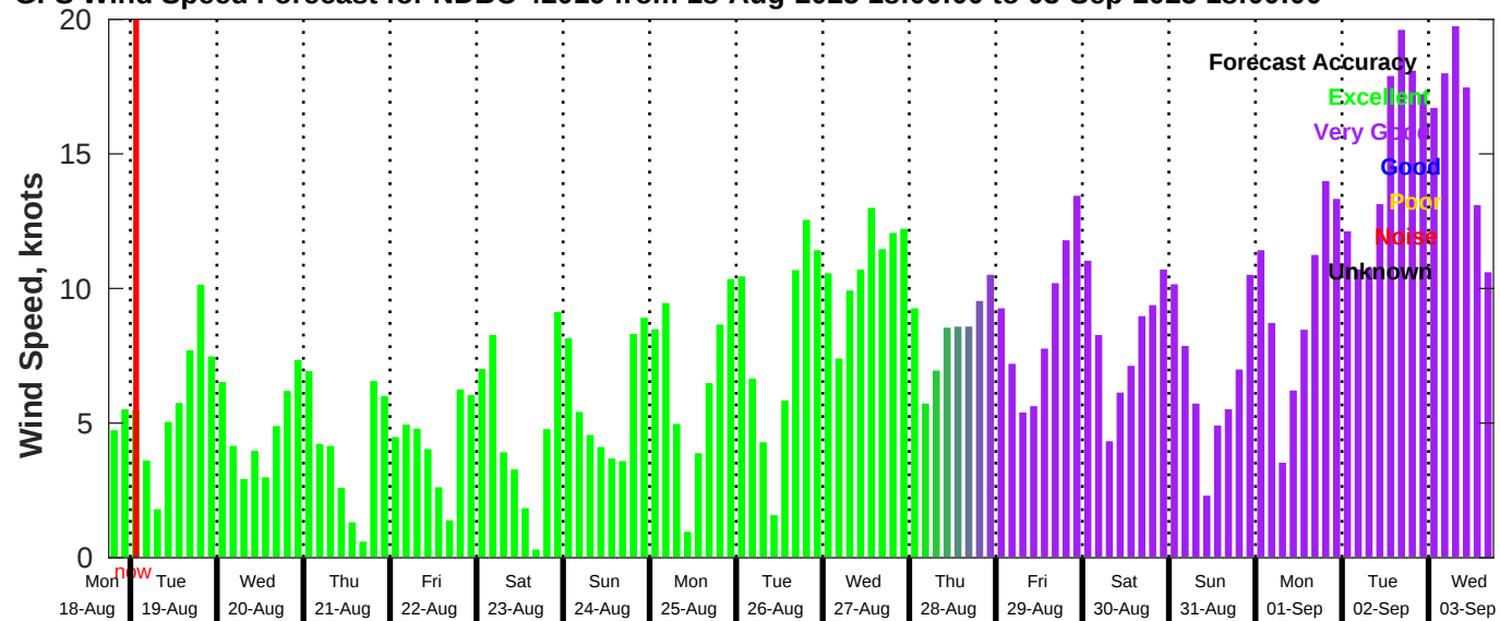
GFS Wind Speed Forecast for NDBC 42019 from 18-Aug-2025 18:00:00 to 03-Sep-2025 18:00:00
