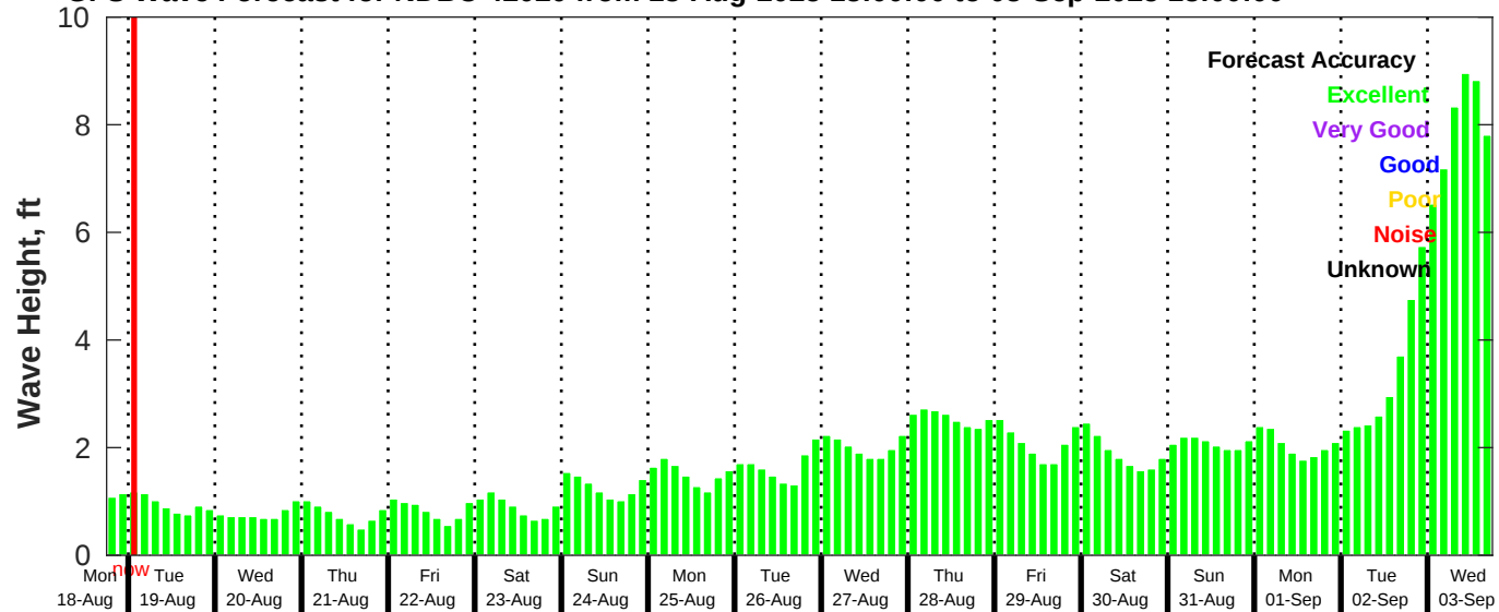
GFS Wave Forecast for NDBC 42020 from 18-Aug-2025 18:00:00 to 03-Sep-2025 18:00:00
