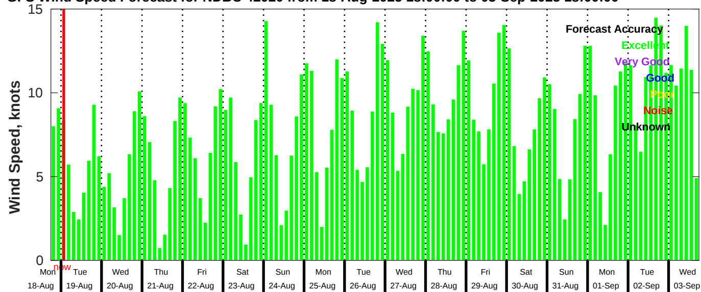
GFS Wind Speed Forecast for NDBC 42020 from 18-Aug-2025 18:00:00 to 03-Sep-2025 18:00:00
