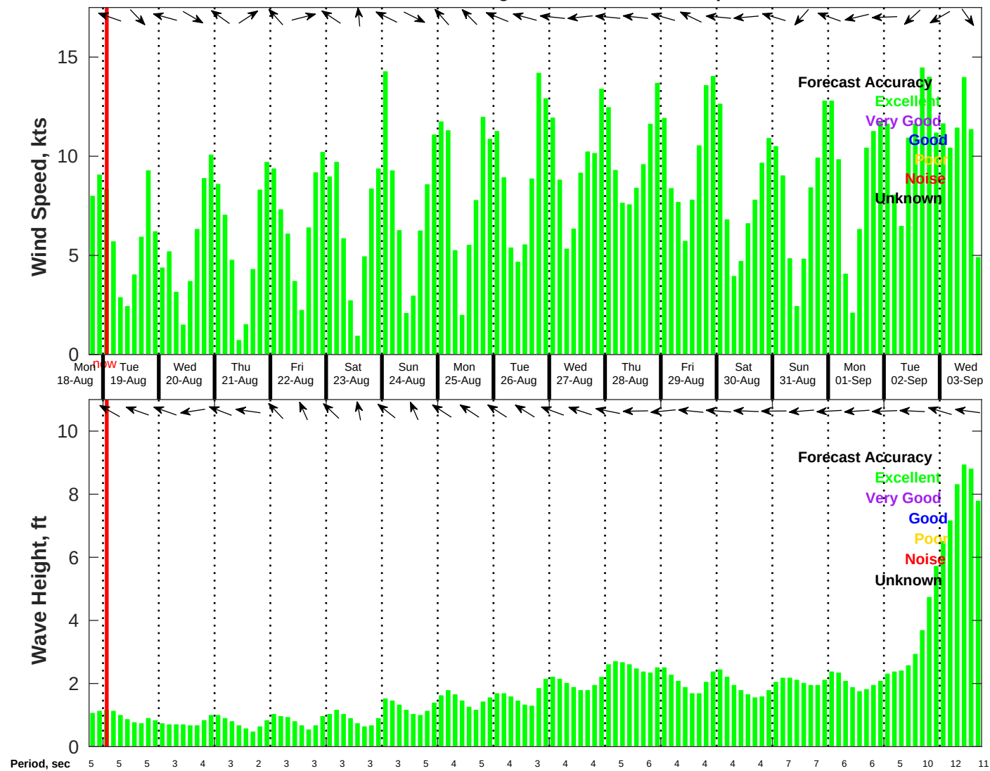
Wind & Wave Forecast for NDBC 42020 from 18-Aug-2025 18:00:00 to 03-Sep-2025 18:00:00
