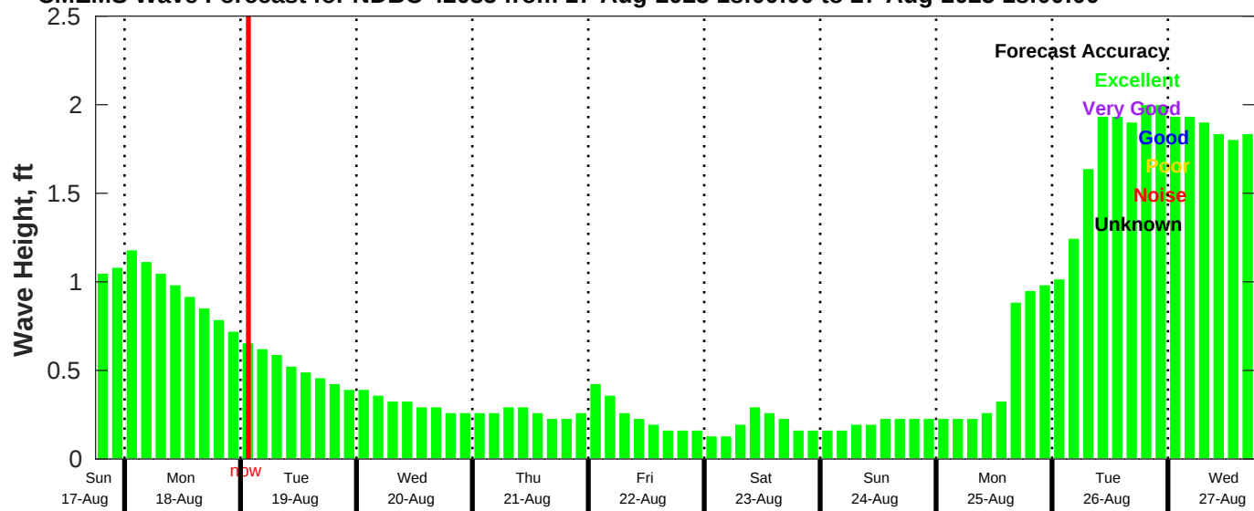
CMEMS Wave Forecast for NDBC 42035 from 17-Aug-2025 18:00:00 to 27-Aug-2025 18:00:00
