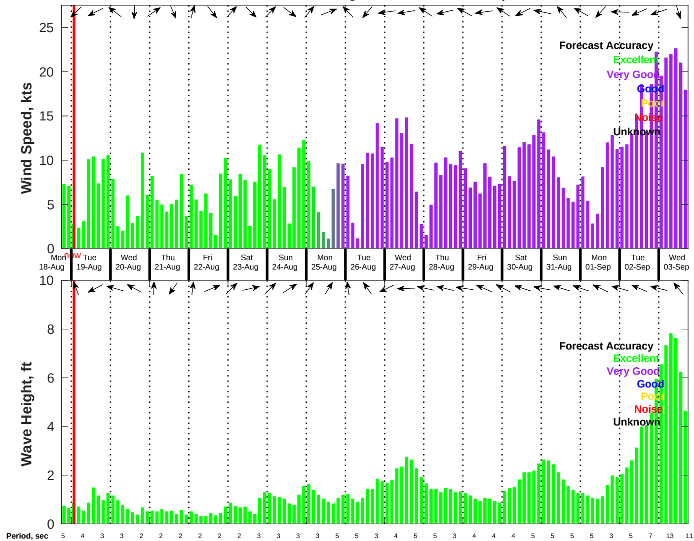
Wind & Wave Forecast for NDBC 42035 from 18-Aug-2025 18:00:00 to 03-Sep-2025 18:00:00
