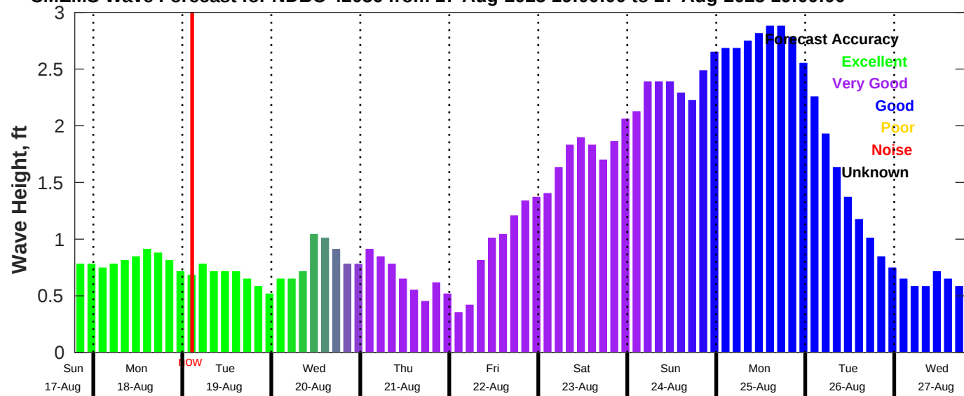
CMEMS Wave Forecast for NDBC 42036 from 17-Aug-2025 19:00:00 to 27-Aug-2025 19:00:00
