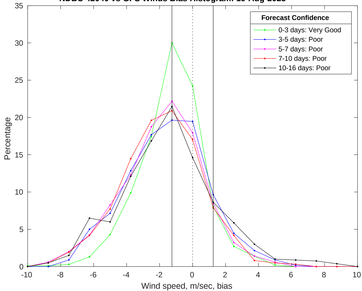
NDBC 42040 vs GFS Winds Bias Histogram: 19-Aug-2025
