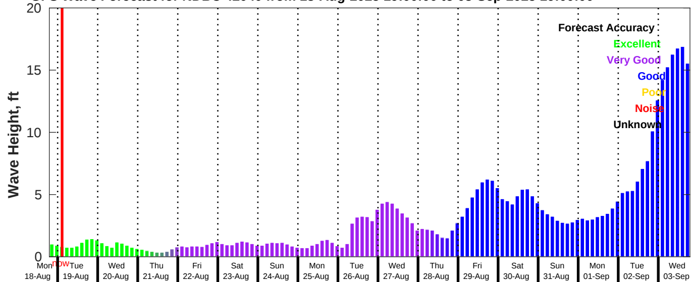
GFS Wave Forecast for NDBC 42040 from 18-Aug-2025 19:00:00 to 03-Sep-2025 19:00:00
